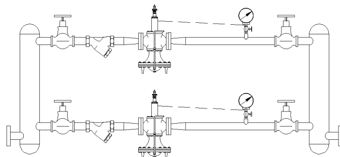
Parallel Unit w/ Manufactured Manifolds
