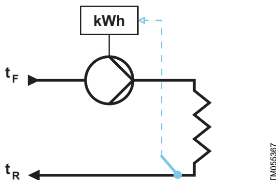
MAGNA3 with built-in heat energy monitor
