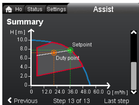
Example of setpoint calculation based on a chosen control mode and entered Q and H values
