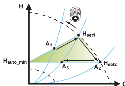
AUTOADAPT control
