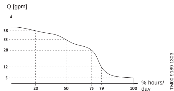
Fig. 8 Duty-time profile
