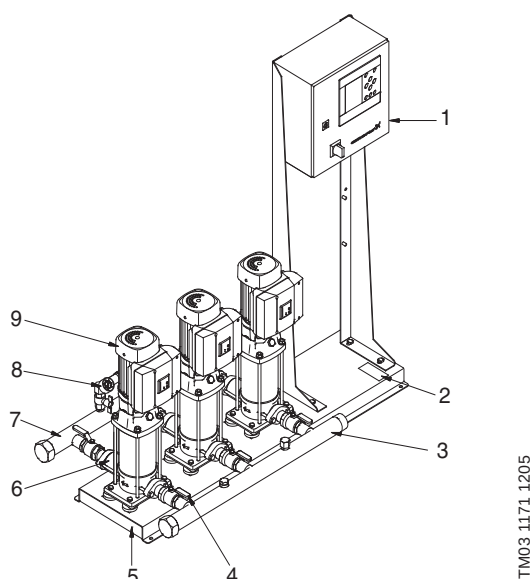
Fig. 4 System components
