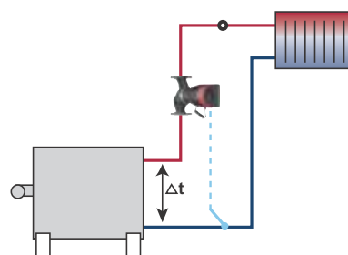
Fig. 32 Differential temperature
