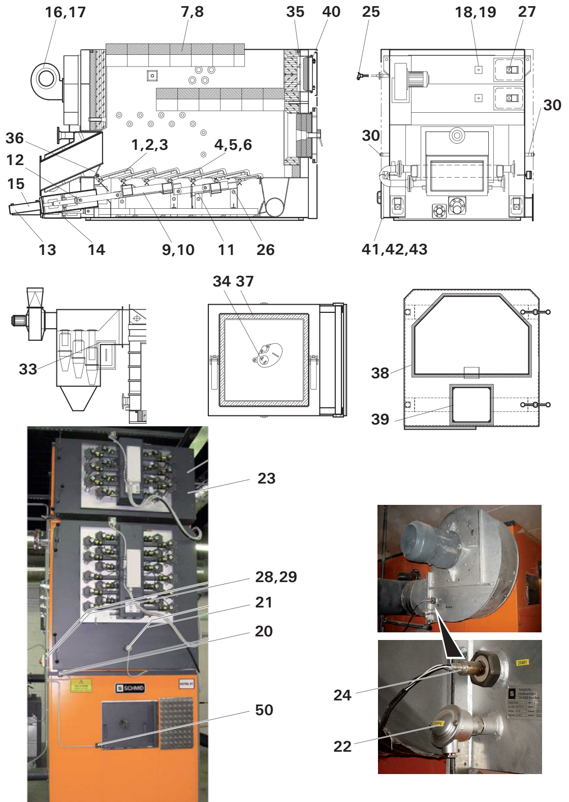
Fig. 22 Spare parts for the UTSR moving grate combustion system
