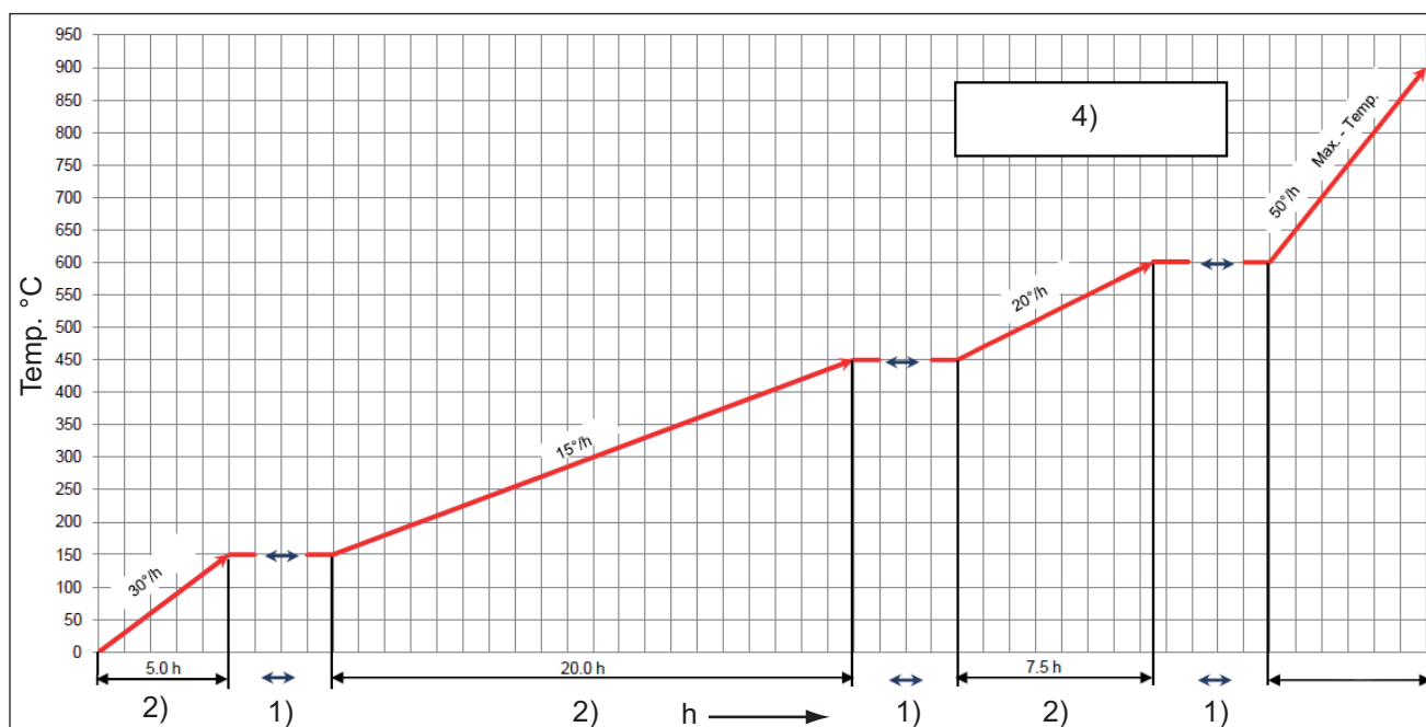
Fig. 17 Heating curve
