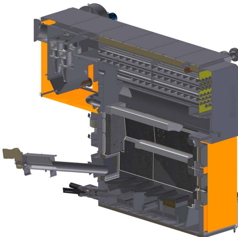
Fig. 3 Cross-section of the moving grate combustion system
