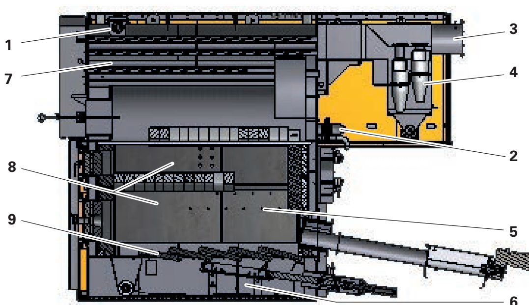
Fig. 4 Basic construction
