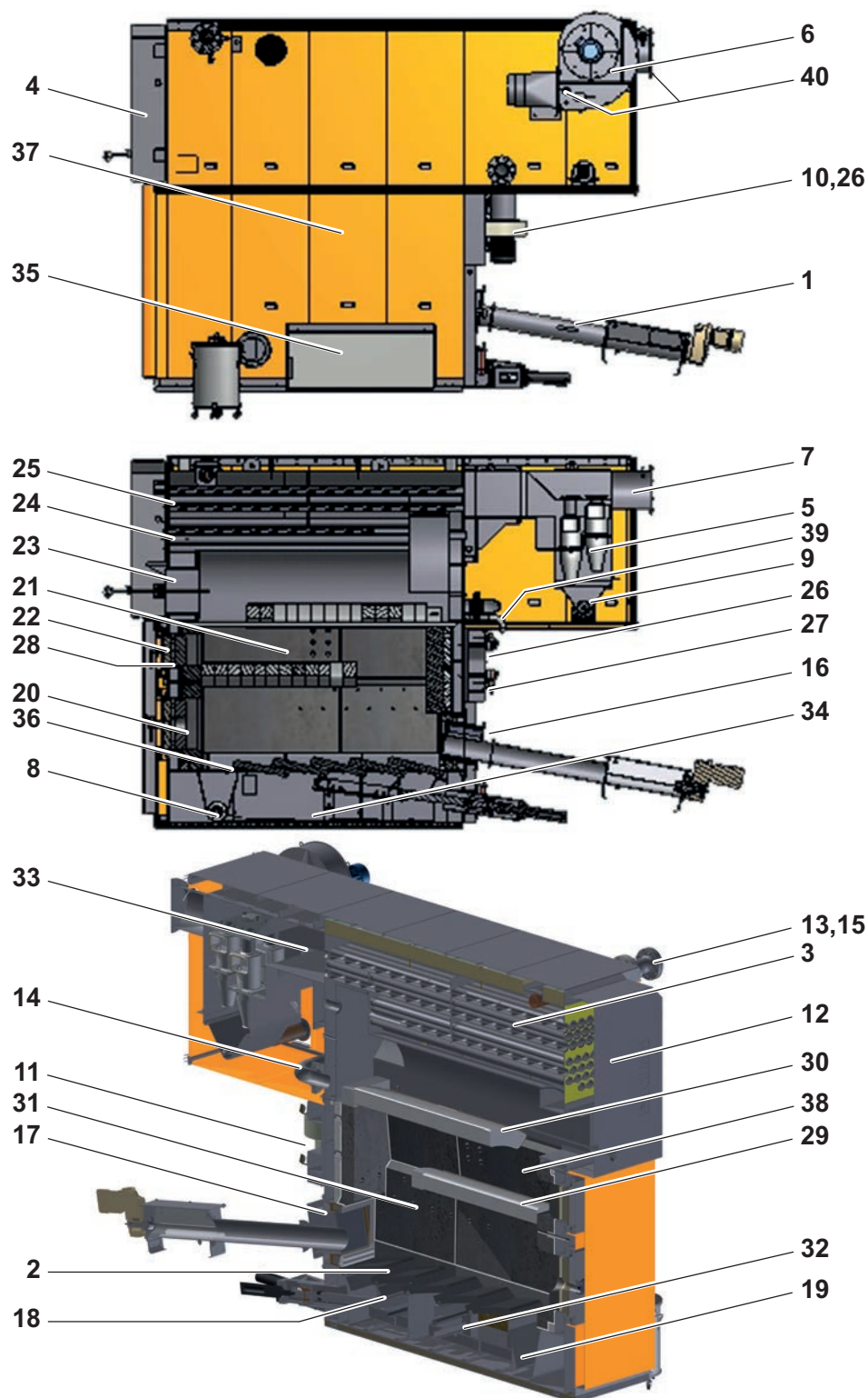
Fig. 5 Design of the moving grate combustion system
