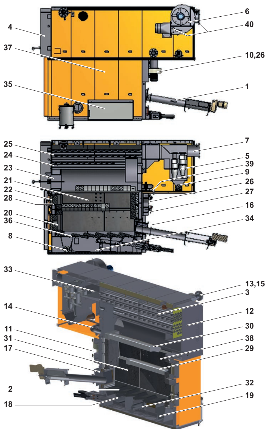
Fig. 19 Maintenance overview
