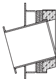
Fig. 13 Inlet design variants
