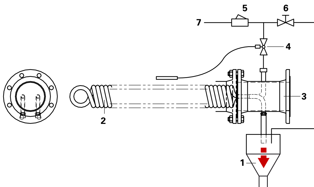
Fig. 9 Temperature safety valve
