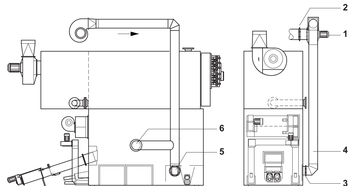
Fig. 26 Flue gas recovery (example illustrated)
