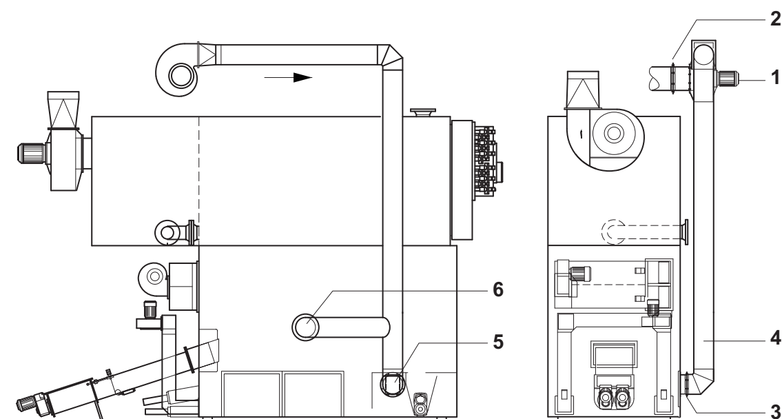
Fig. 10 Flue gas recovery (example illustrated)
