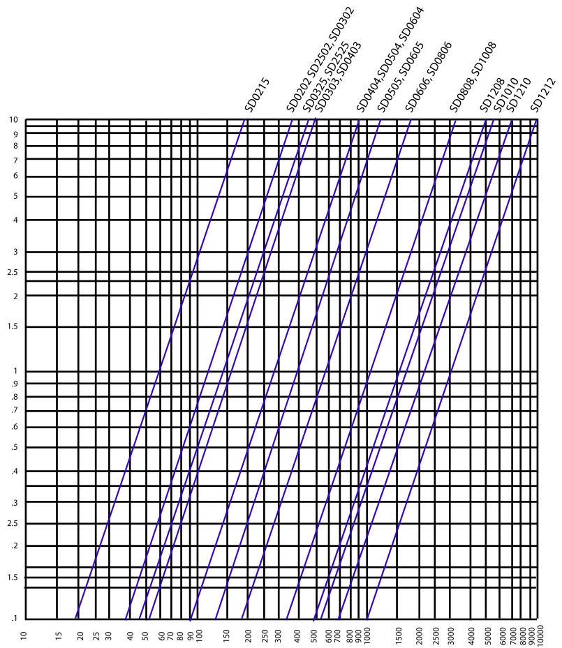
FLOW RATE - GPM WATER AT 70°F
