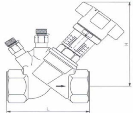
Threaded Connection
